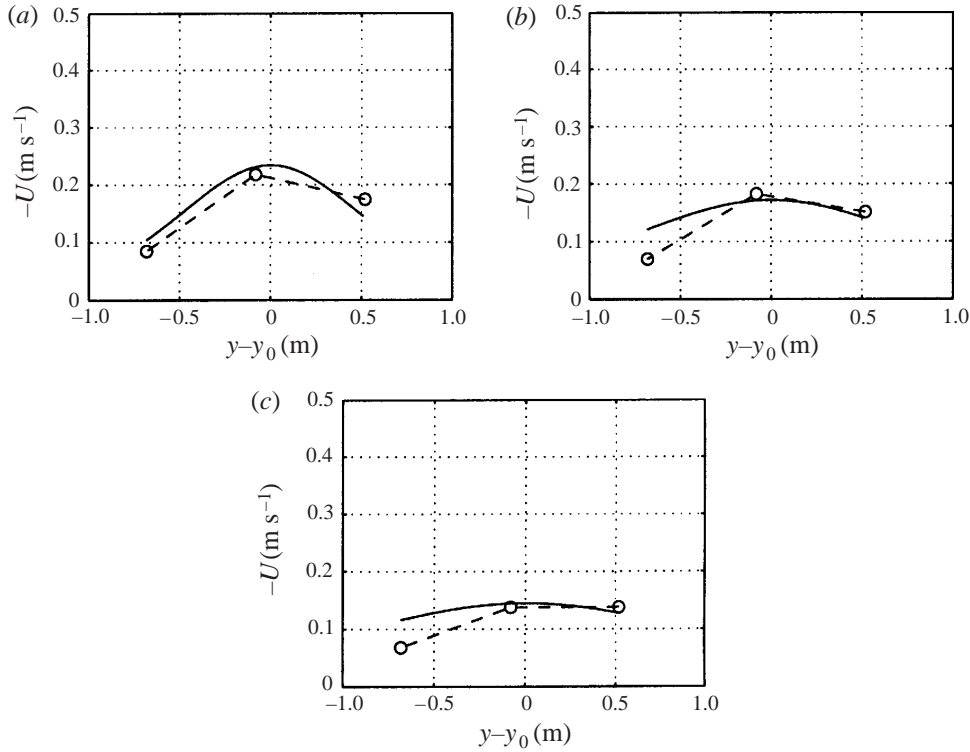
FIGURE 18. Comparison of best-fit mean rip current velocity profile to experimental data for test G (a) x' = 0 m ( x = 11.93 m), (b) x' = 0.3 m ( x = 11.63 m), (c) x' = 0.5 m ( x = 11.43 m).
